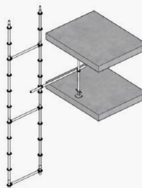
Strut fixing 2
